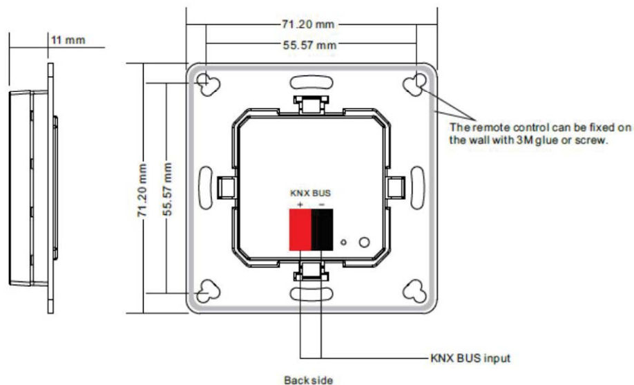
Back side
